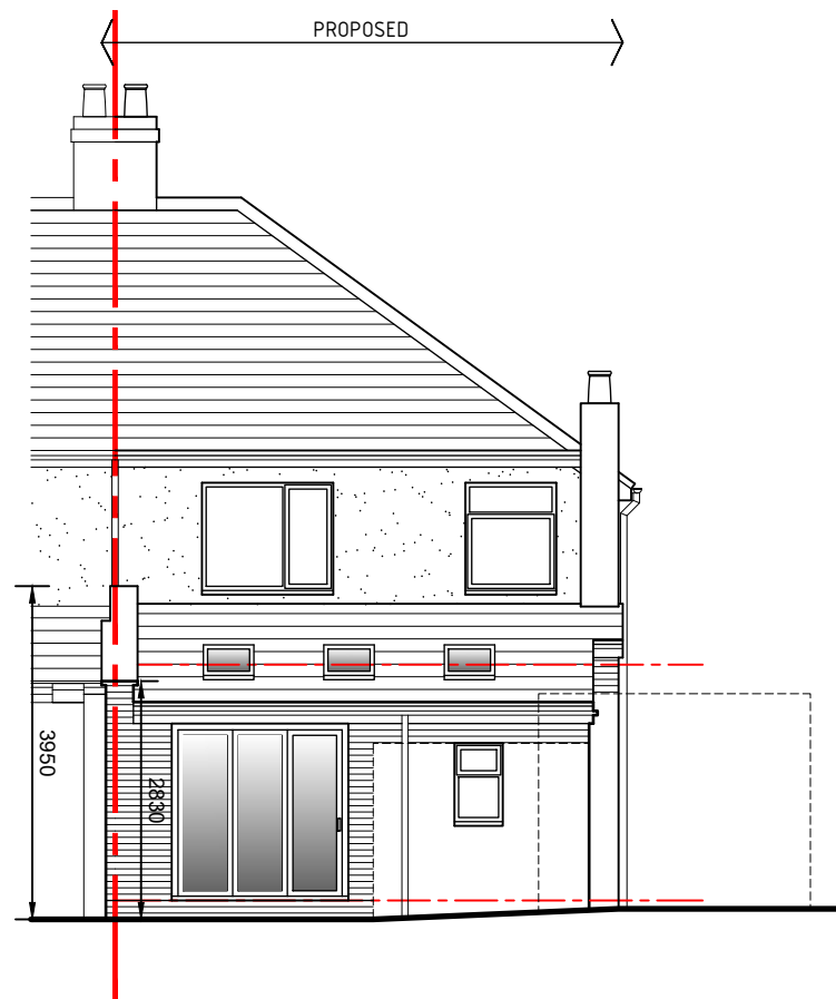
Rear elevation 1:100
