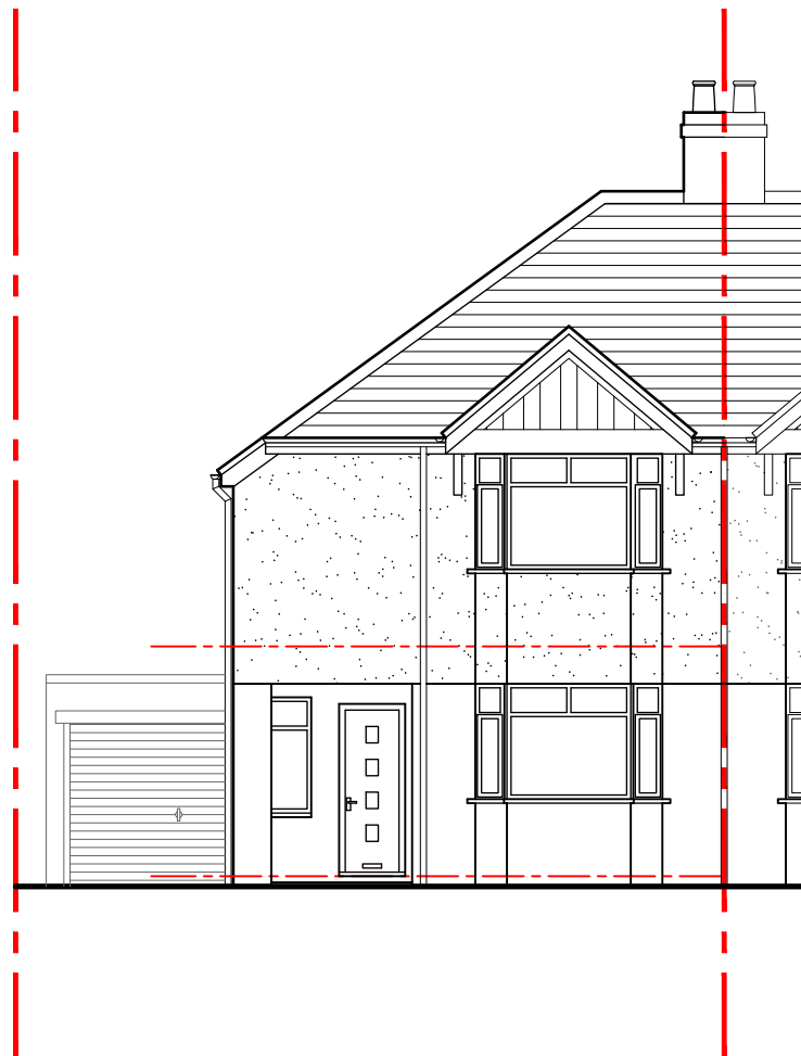
Front elevation 1:100
