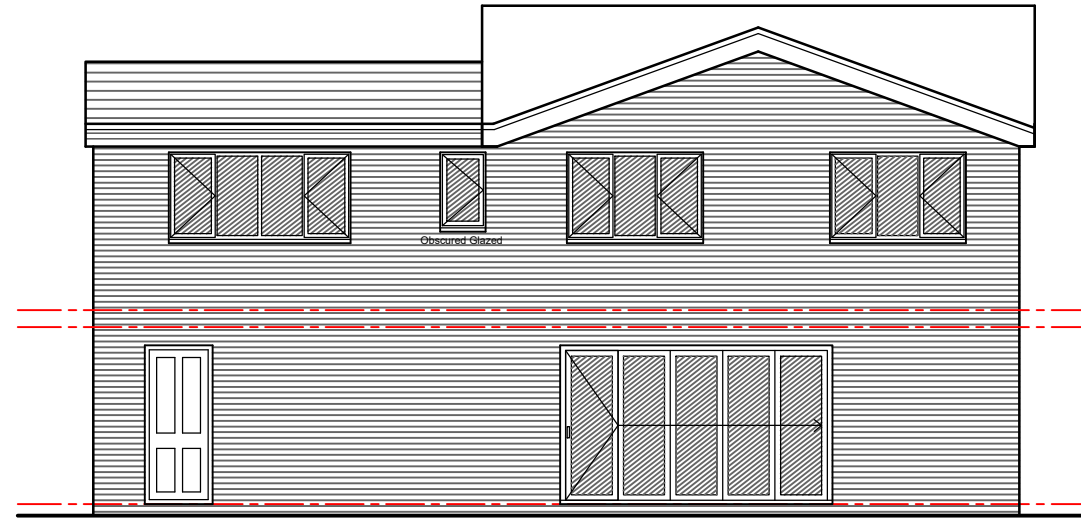
Rear Elevation
