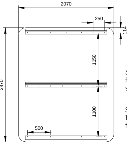
Fixing details For Signage
