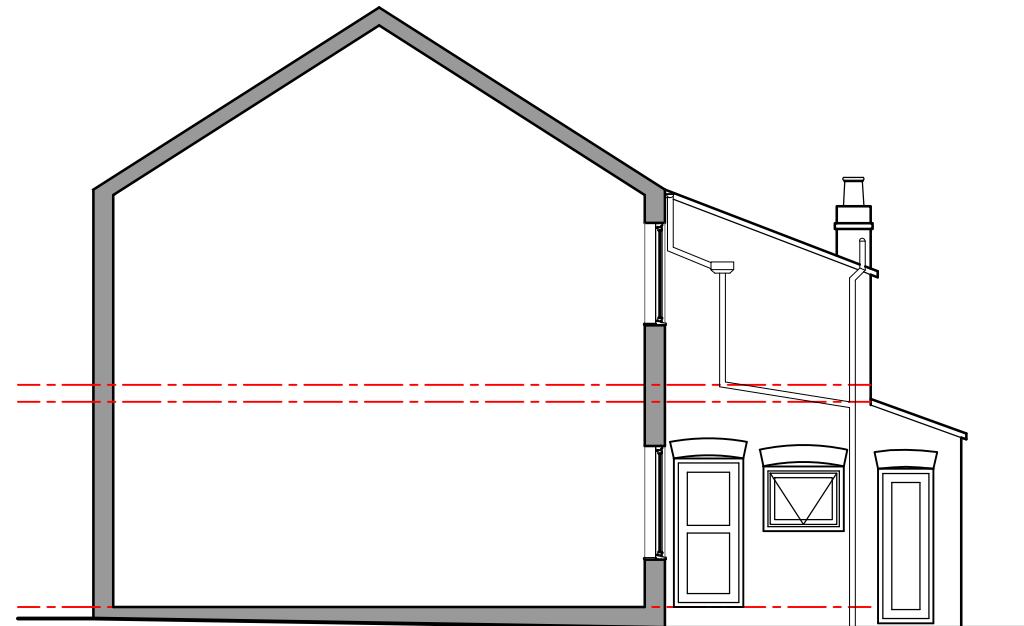
Side 01 Elevation
