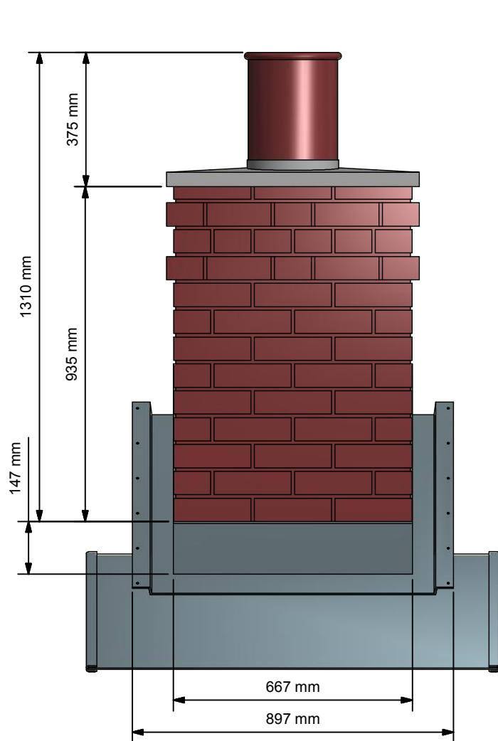
Front Elevation ( 1 : 15 )
