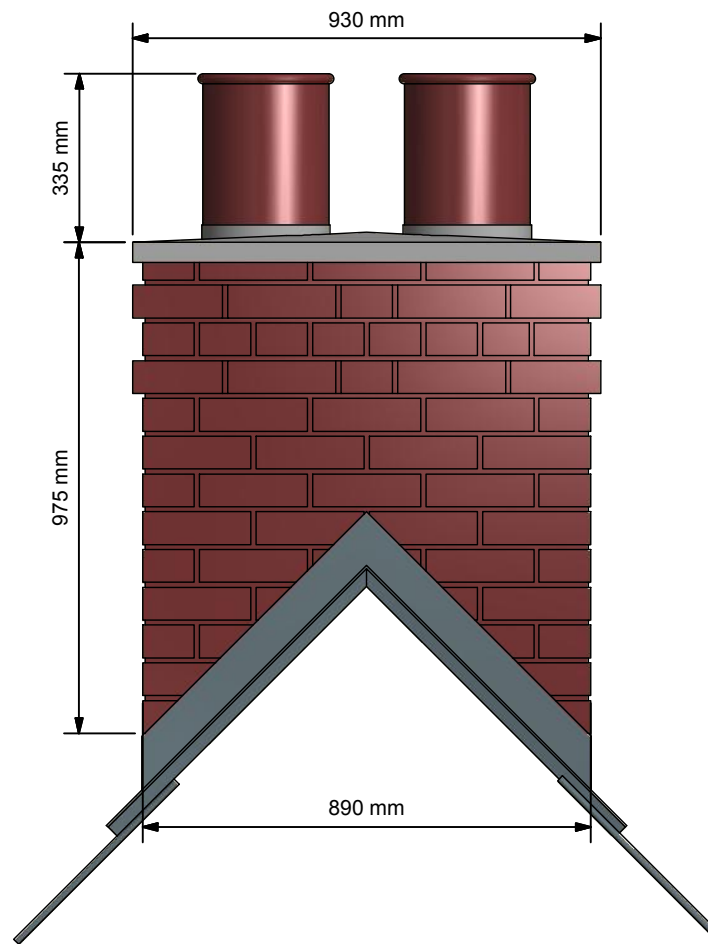
Side Elevation
