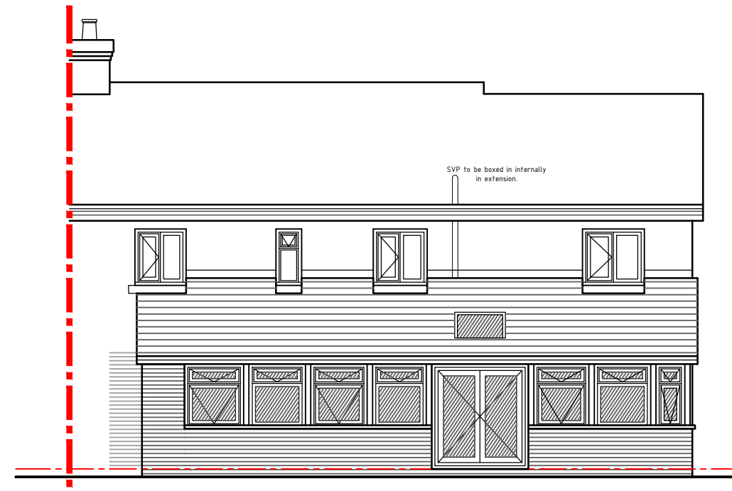
Rear Elevation
