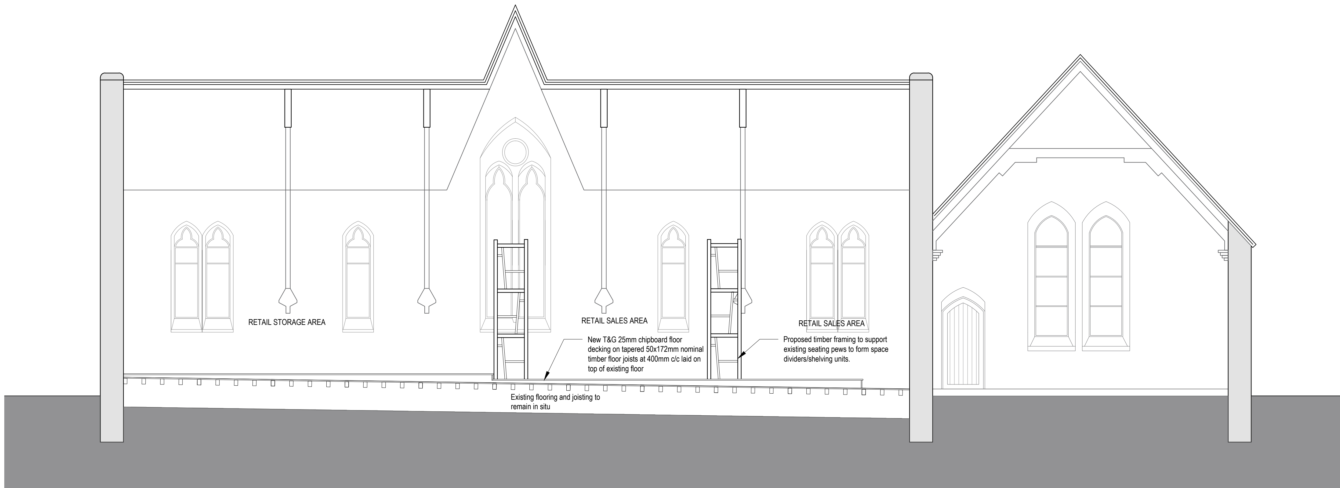
PROPOSED SECTION - 1:50
