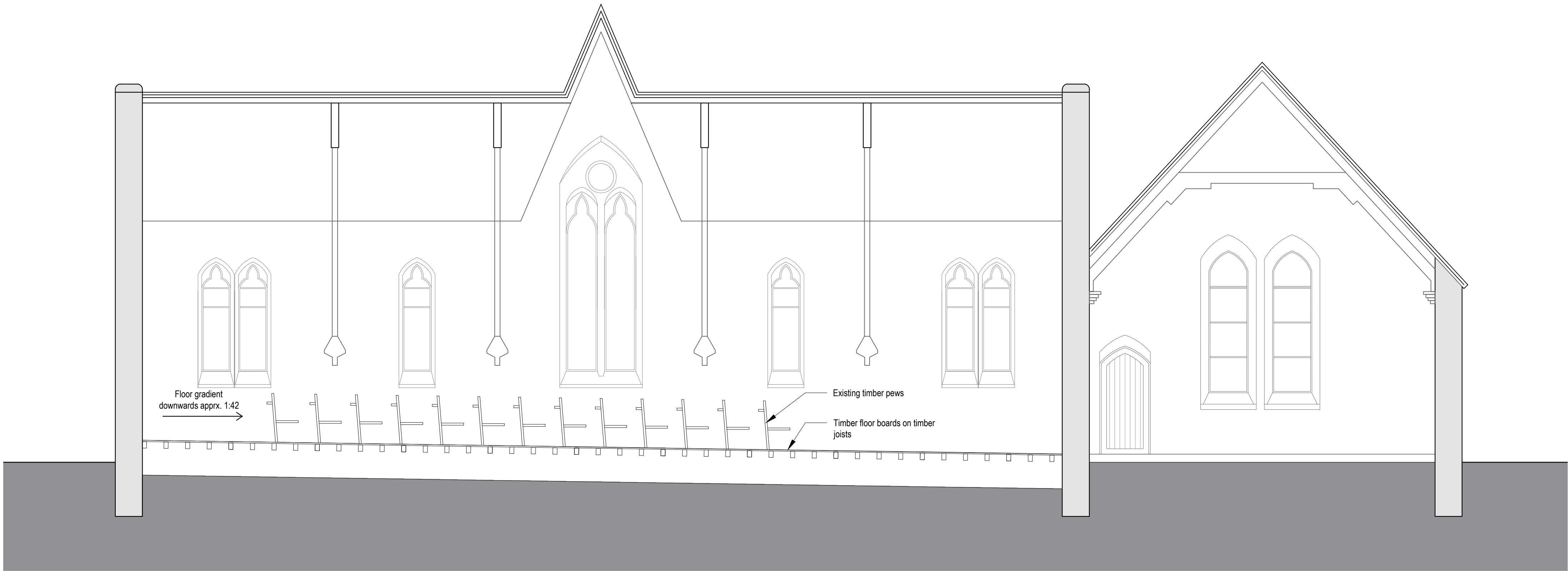
EXISTING SECTION - 1:50
