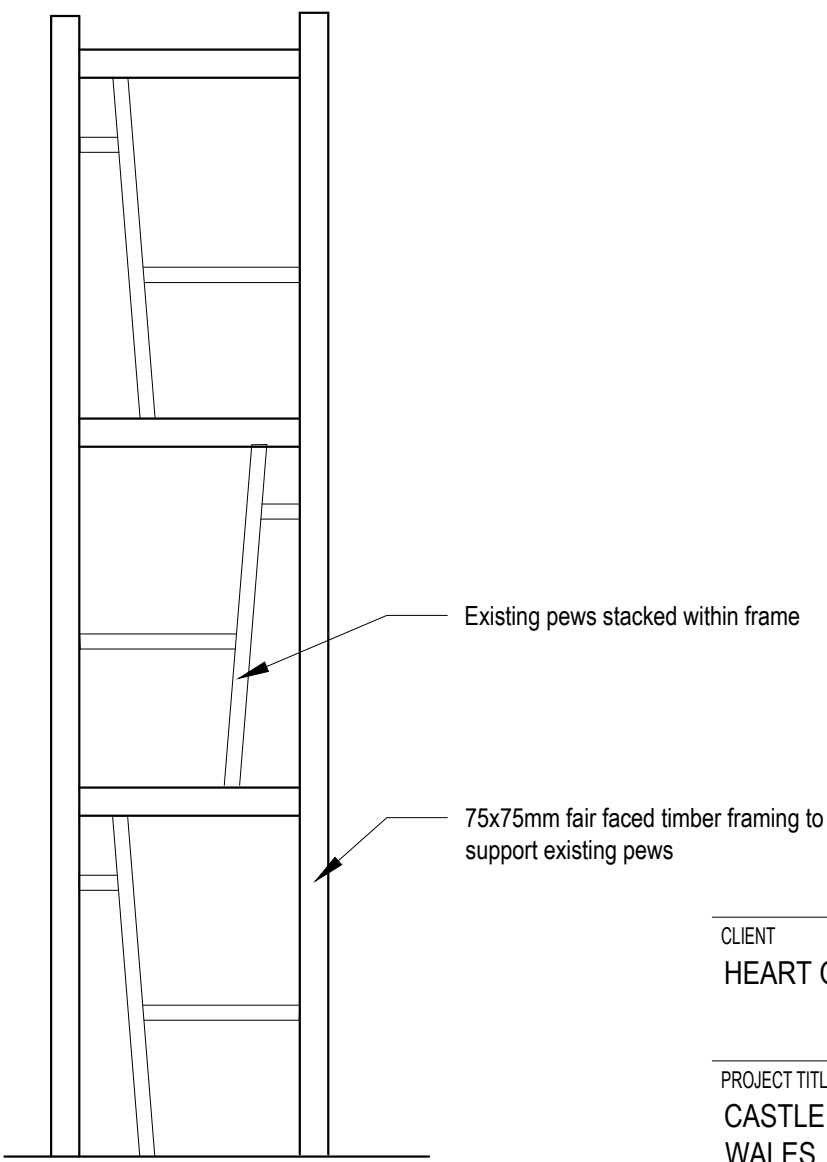
PROPOSED SPACE DIVIDERS/SHELVING - 1:20
