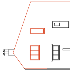
Proposed South Side Elevation
