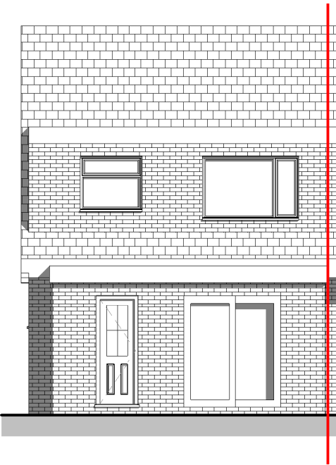
Rear Elevation 1 : 100
