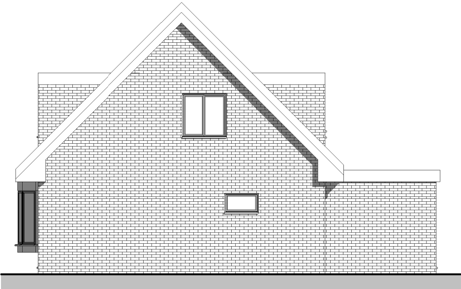
Side Elevation 1 : 100
