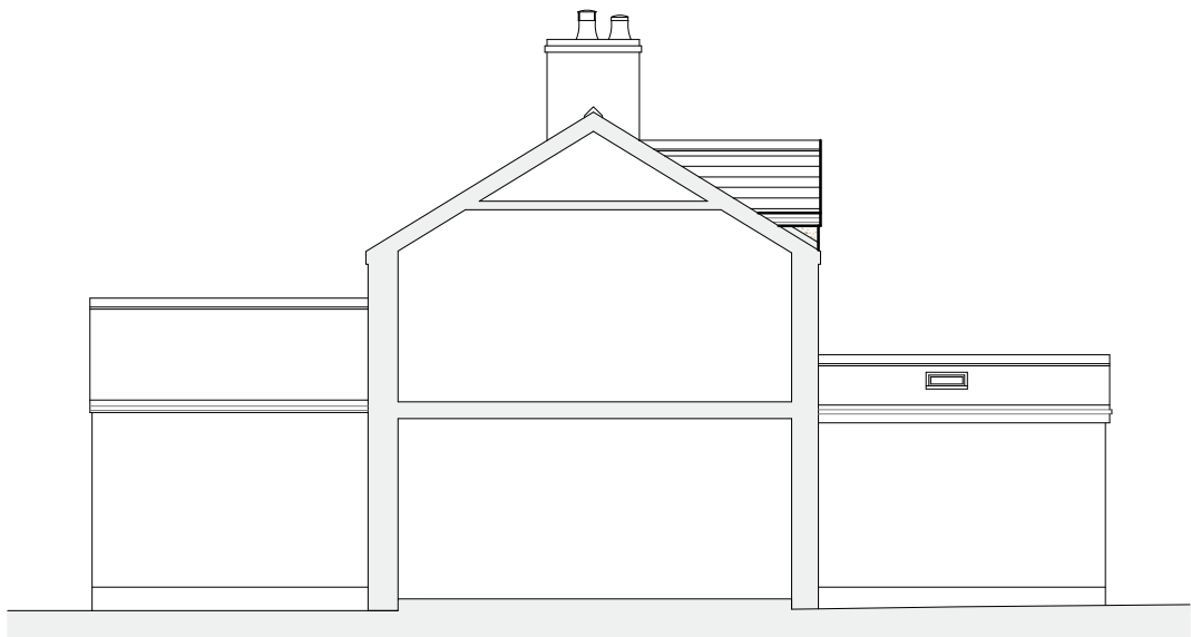
Side Elevation/ Section 1:100
