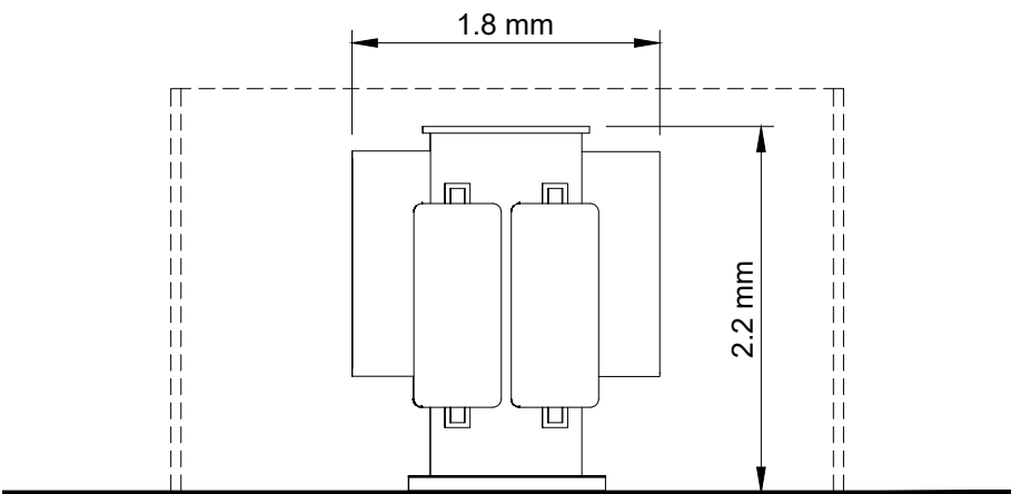
Side
