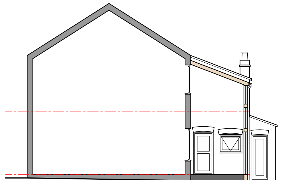
Side 01 Elevation
