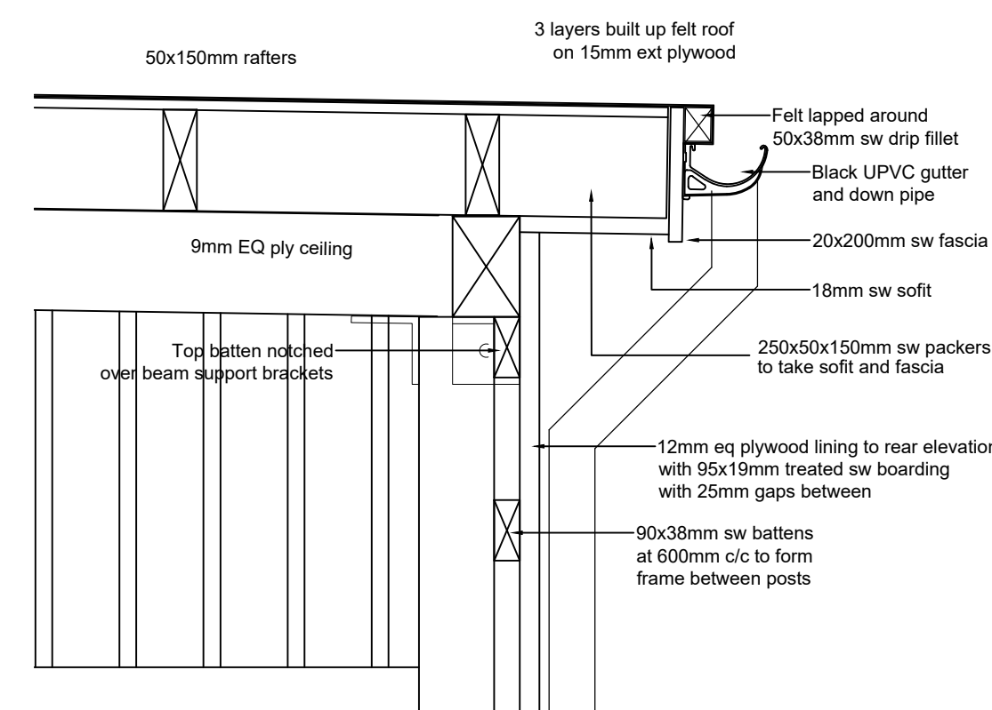
Detail 2 @ 1/10
