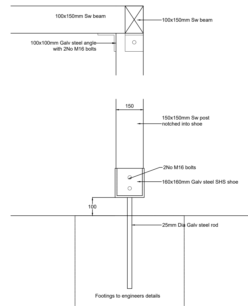
FRAME DETAIL & SECTION 1:10
