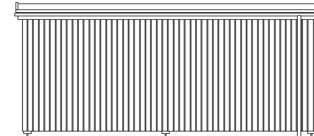
REAR ELEVATION
