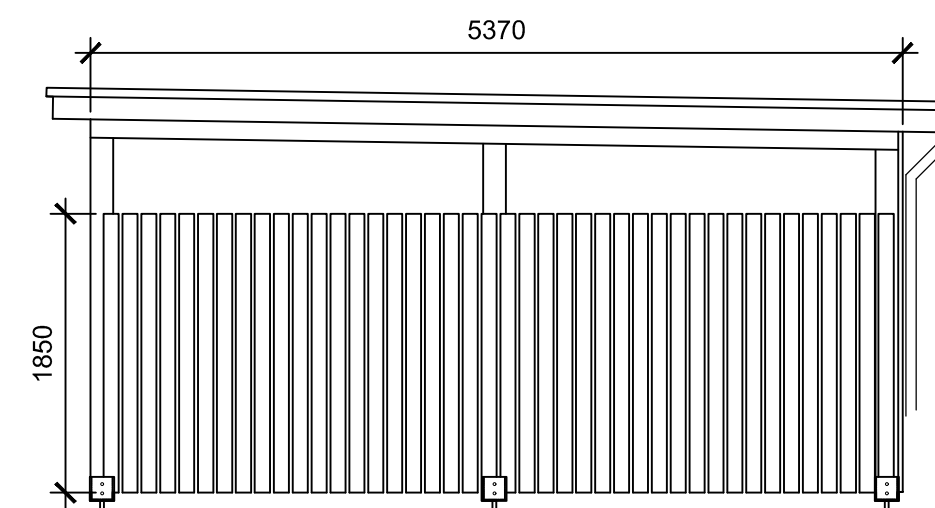
SIDE ELEVATION ( Reception side)
