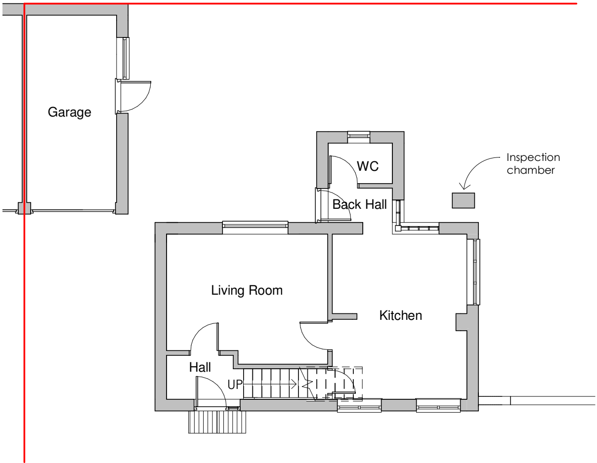
Ground Floor 1 : 100
