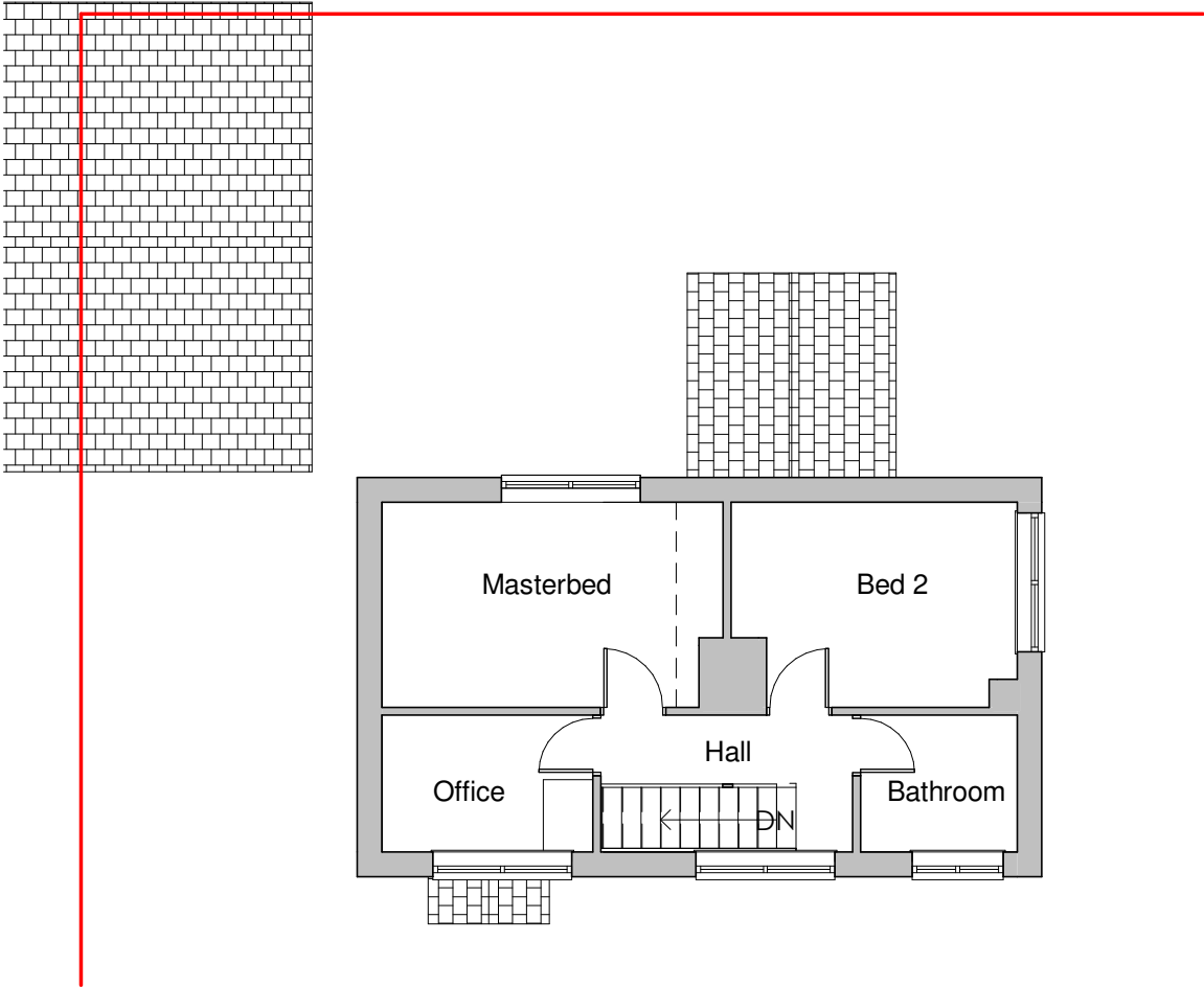
First Floor 1 : 100
