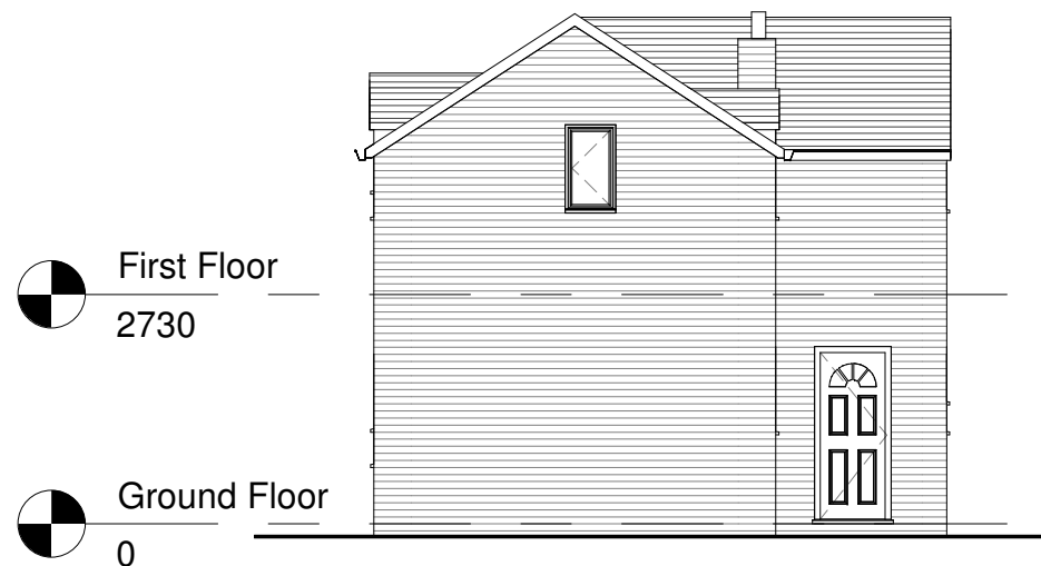
NE (Front) Elevation 1 : 100
