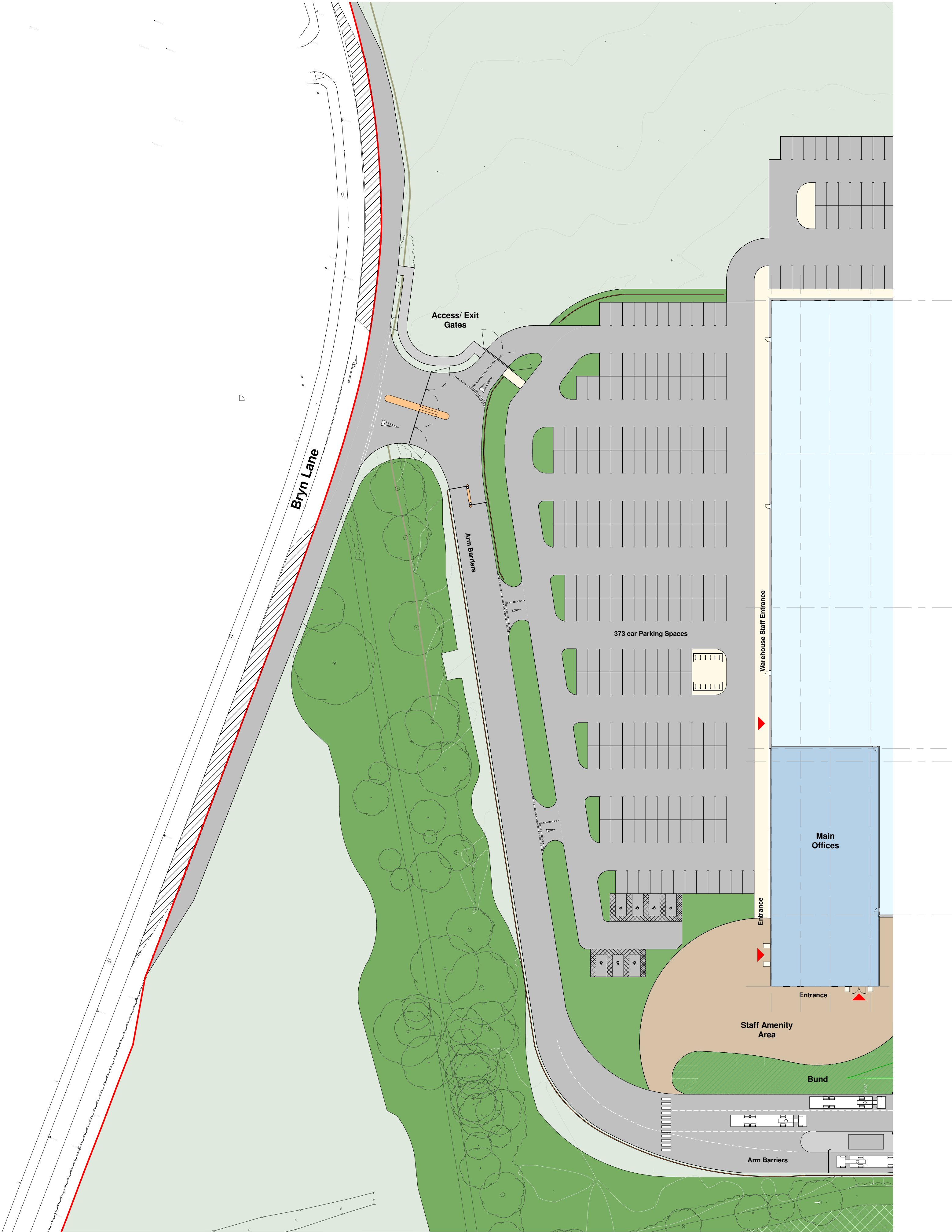
1 Proposed Site Access Plan 1:500
