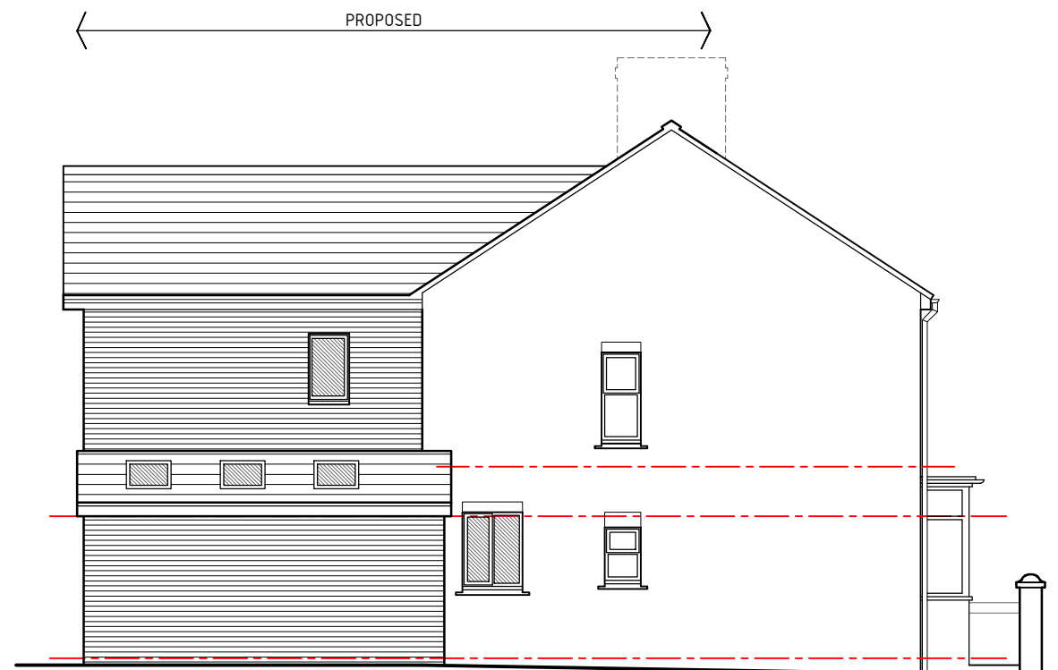
Side-01 Elevation 1:100
