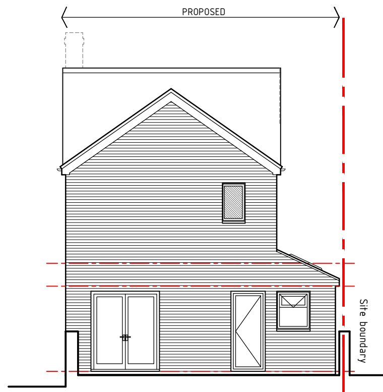
Rear Elevation 1:100
