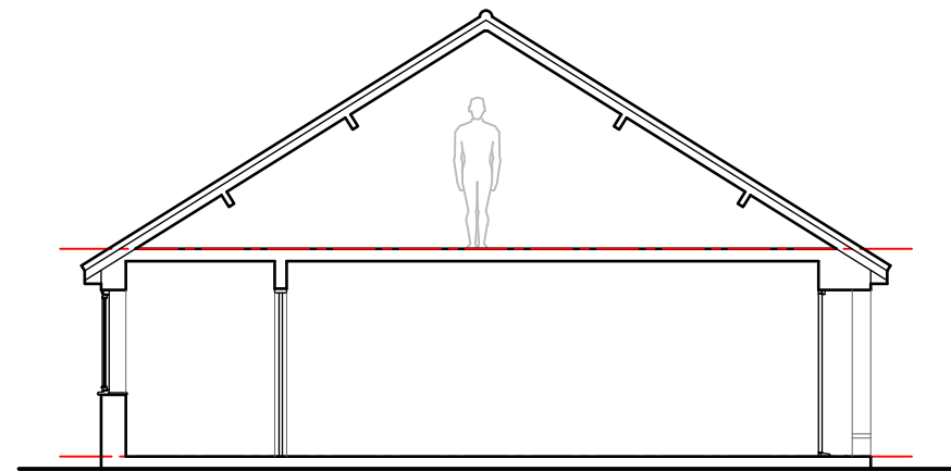
Typical section 1:100
