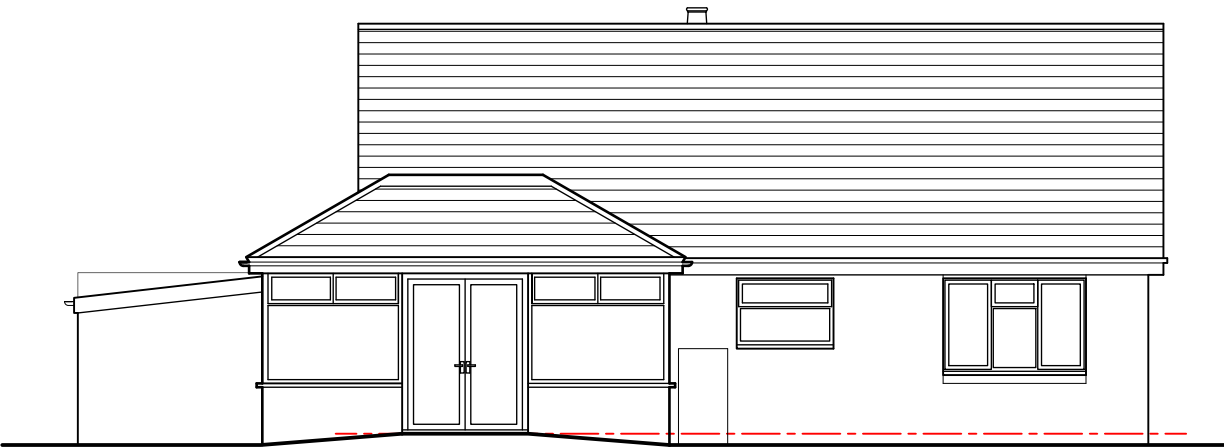
Rear Elevation 1:100
