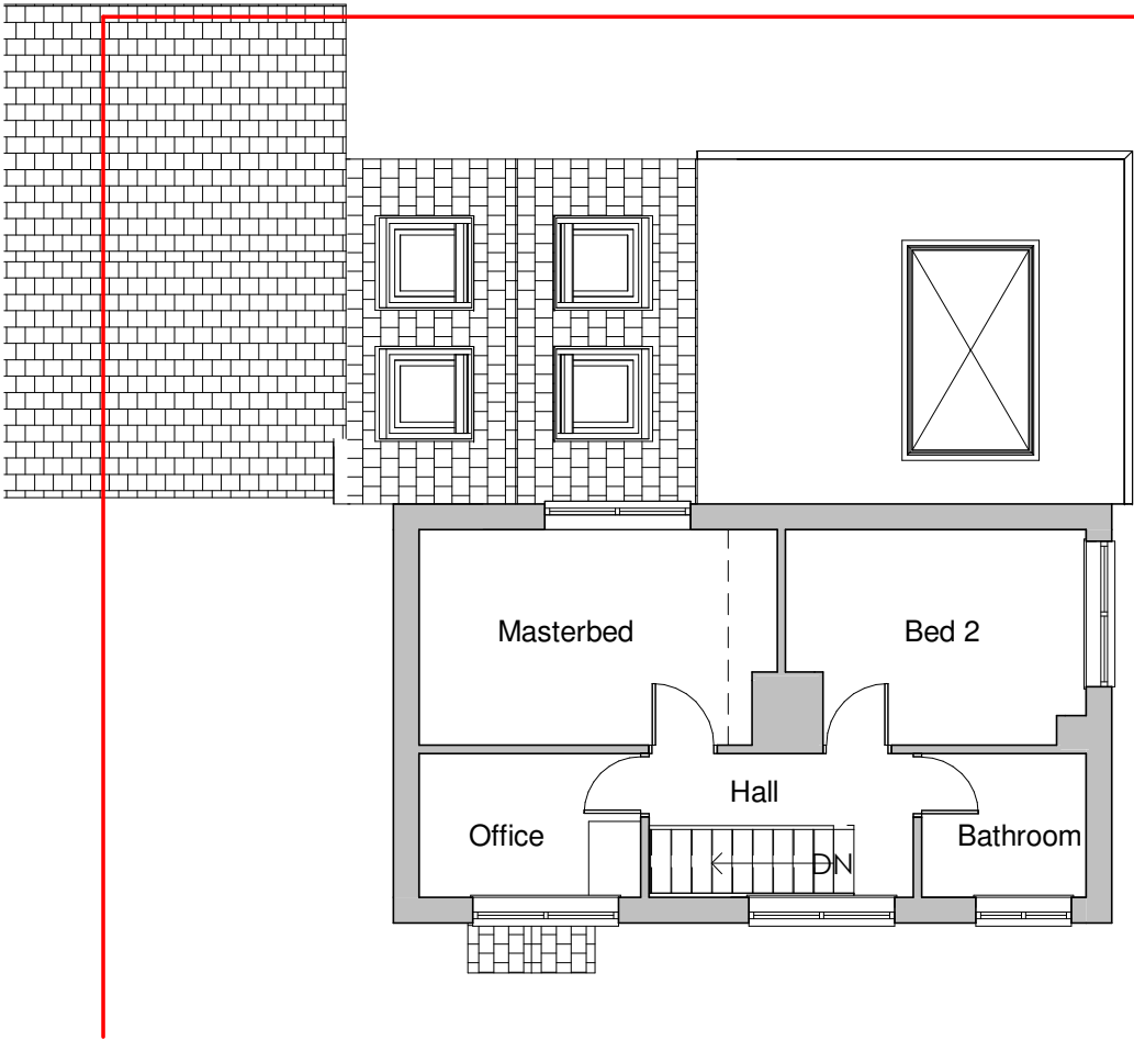
First Floor 1 : 100
