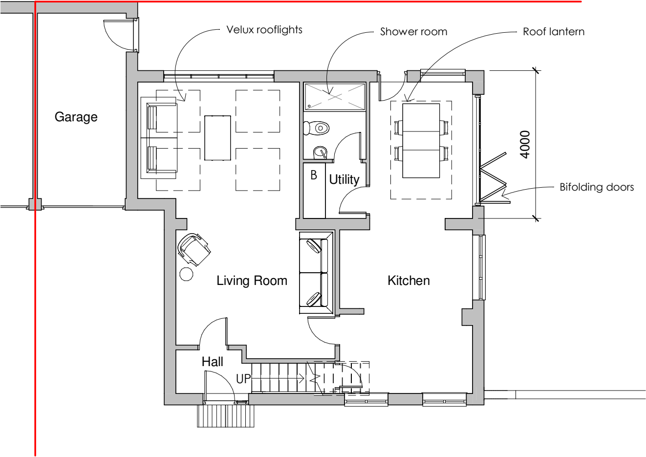
Ground Floor 1 : 100
