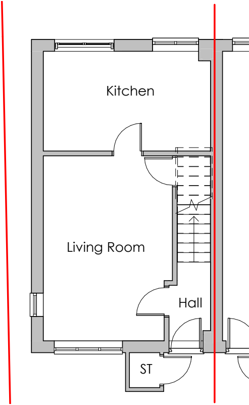
Ground Floor 1 : 100
