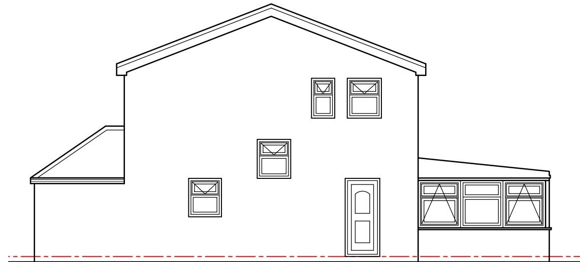
Side 01 Elevation
