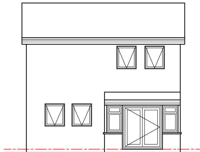
Rear Elevation
