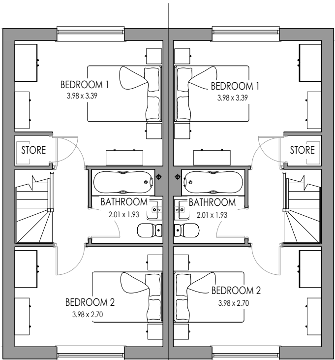
OAKLEY AS FIRST FLOOR
