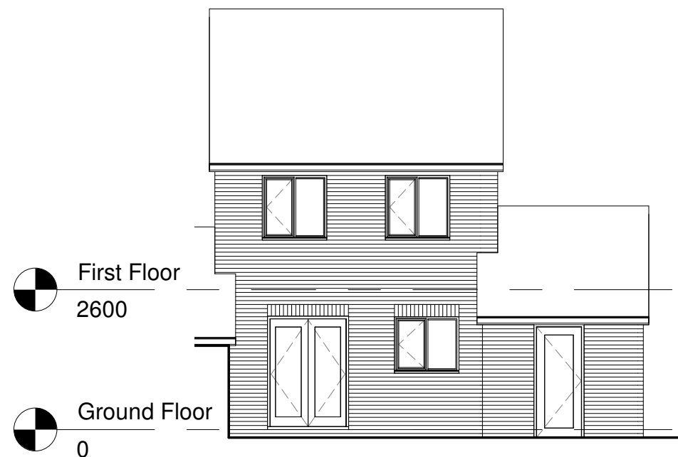
South 1 : 100
