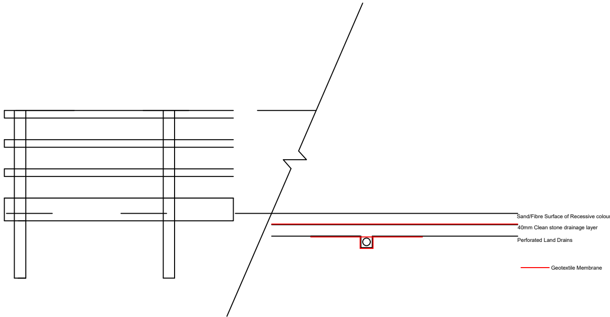
1:50 Typical Sections
