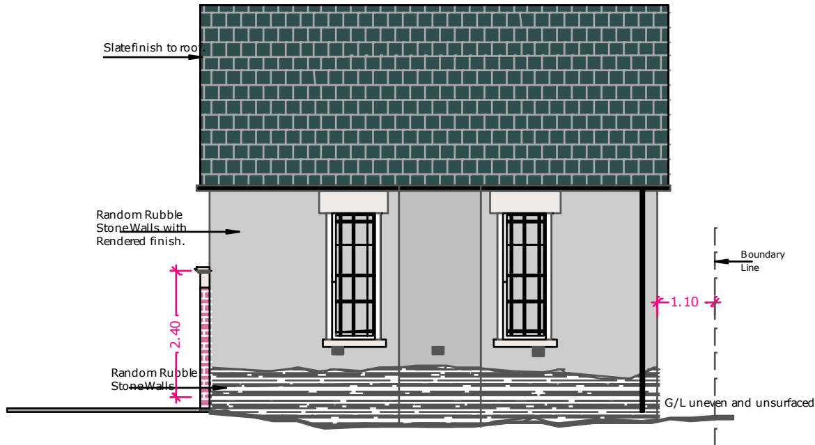
Existing North West Elevation - 1:100
