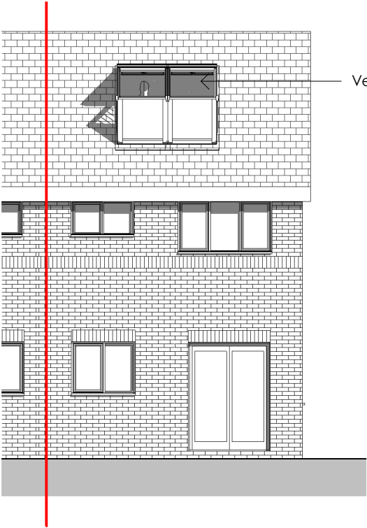
Rear Elevation 1 : 100
