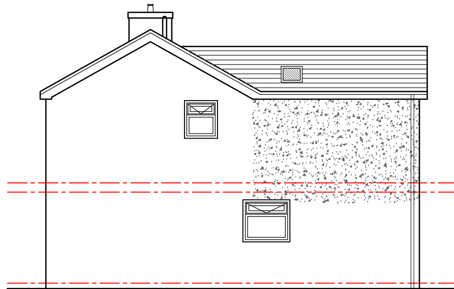
Side 01 Elevation
