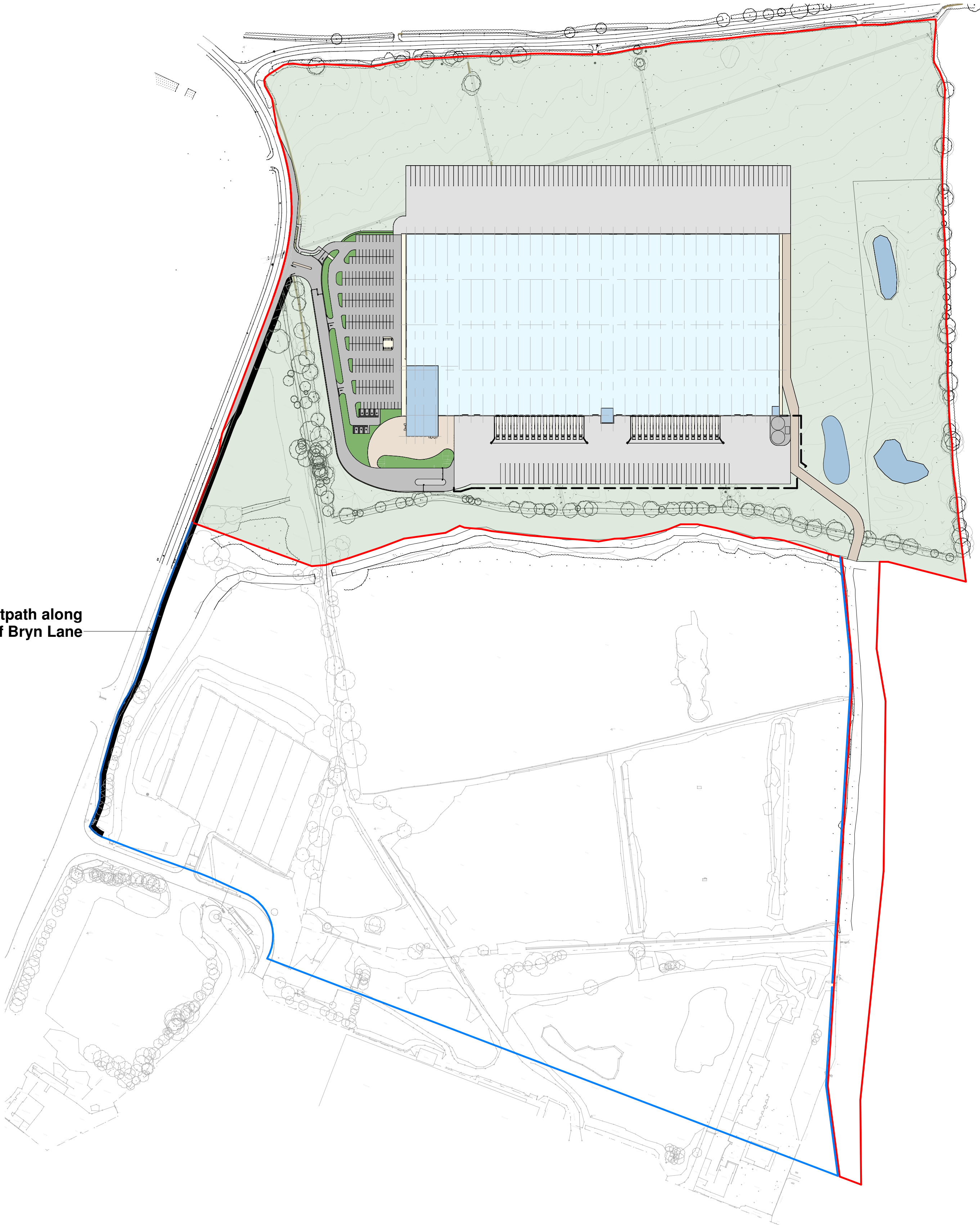
1 Revised Figure 12 1 : 2000
