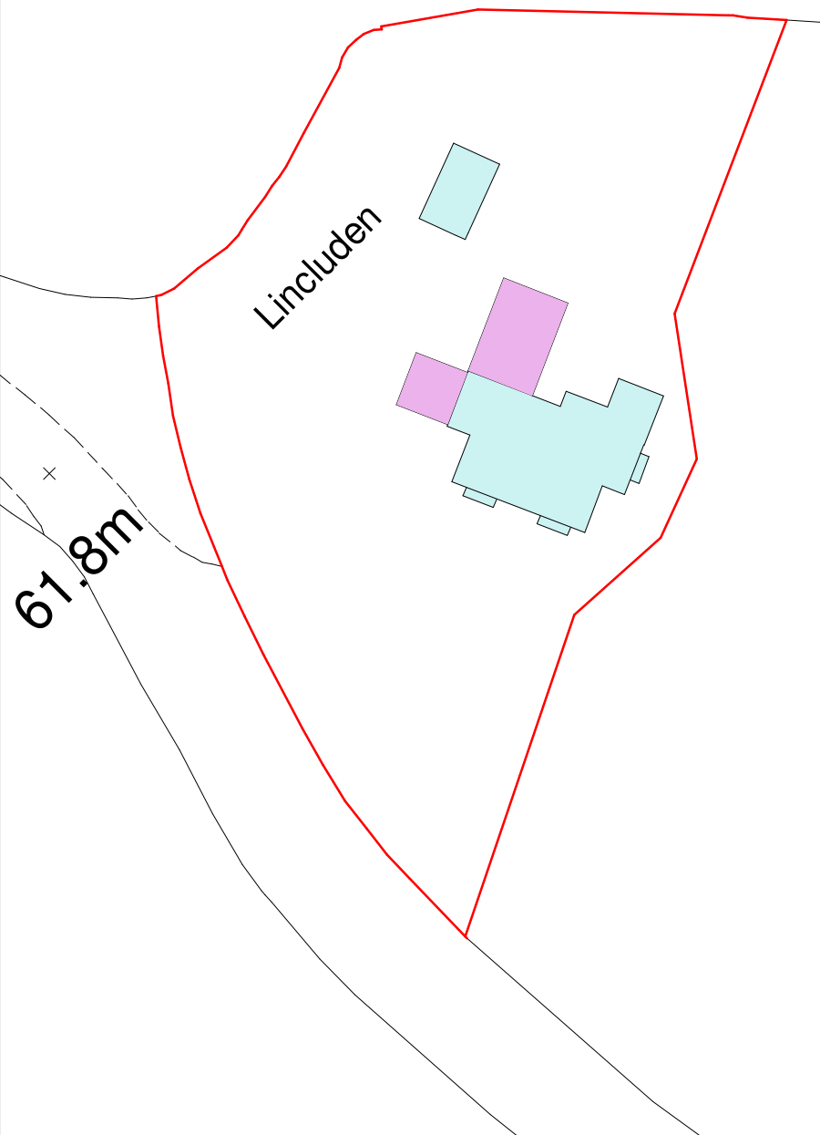
2 PROPOSED SITE PLAN 1 : 500
