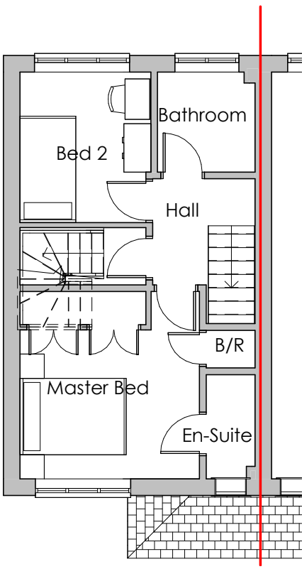
First Floor 1 : 100
