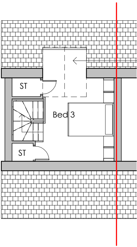
Second Floor 1 : 100
