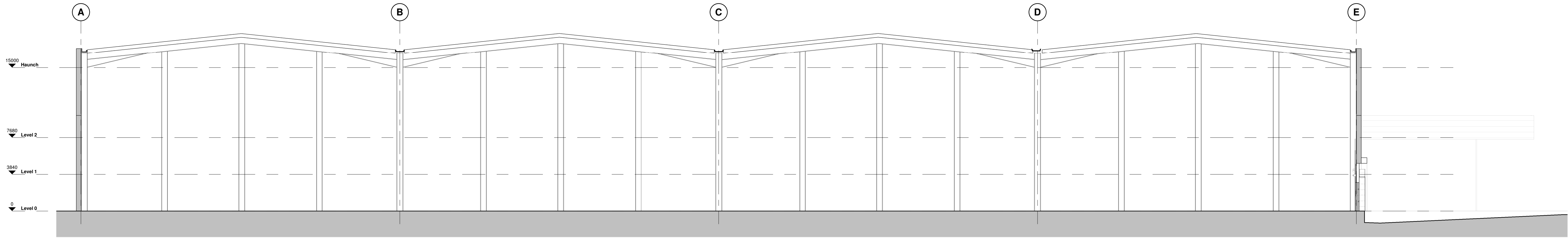
GA-A GA Section A 1 : 200
