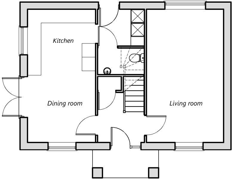
Ground floor layout plan Floor area: 49.9 q m/537 sq ft
