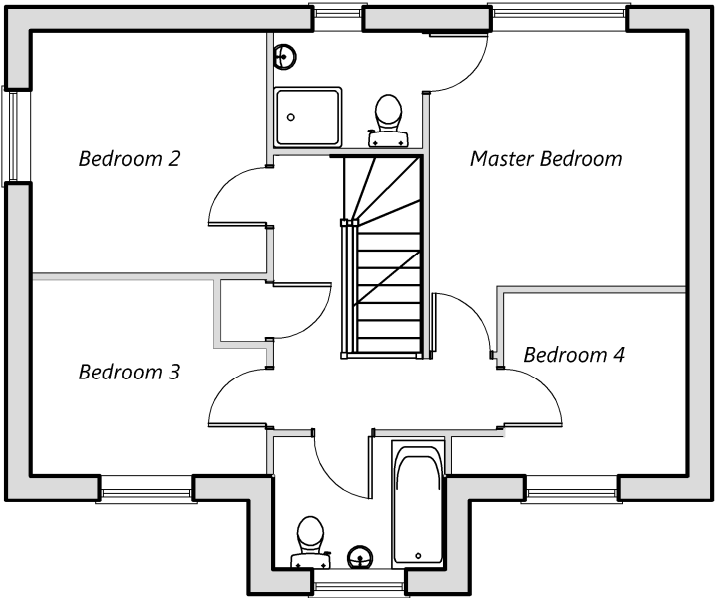
First floor layout plan Floor area: 52.6 q m/566 sq ft
