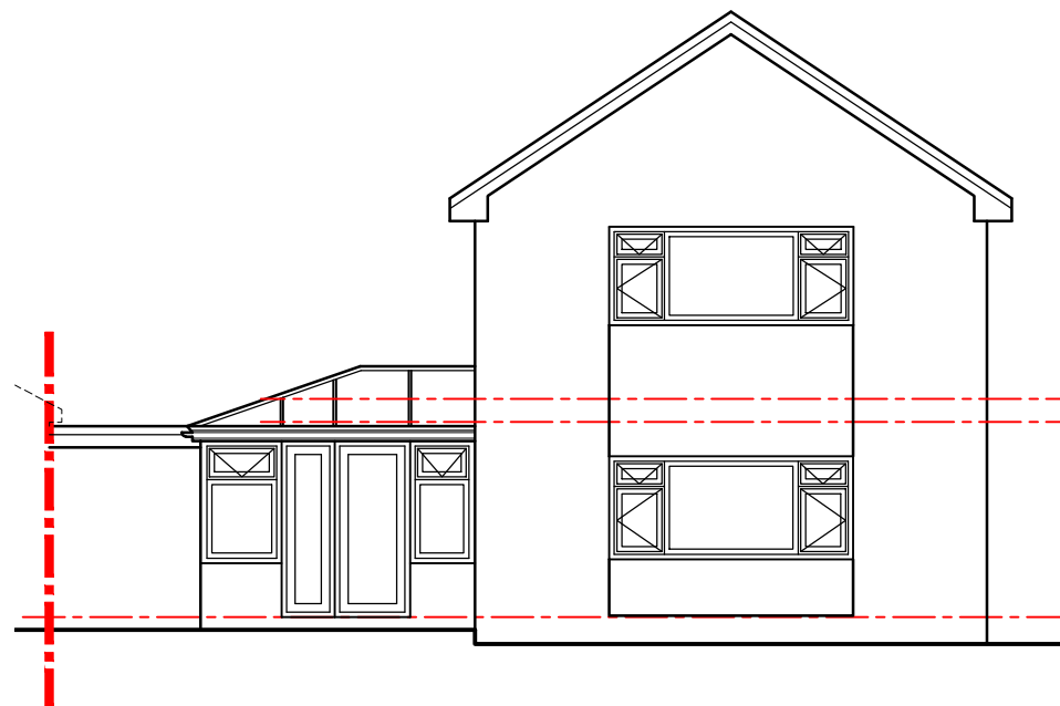
Rear Elevation
