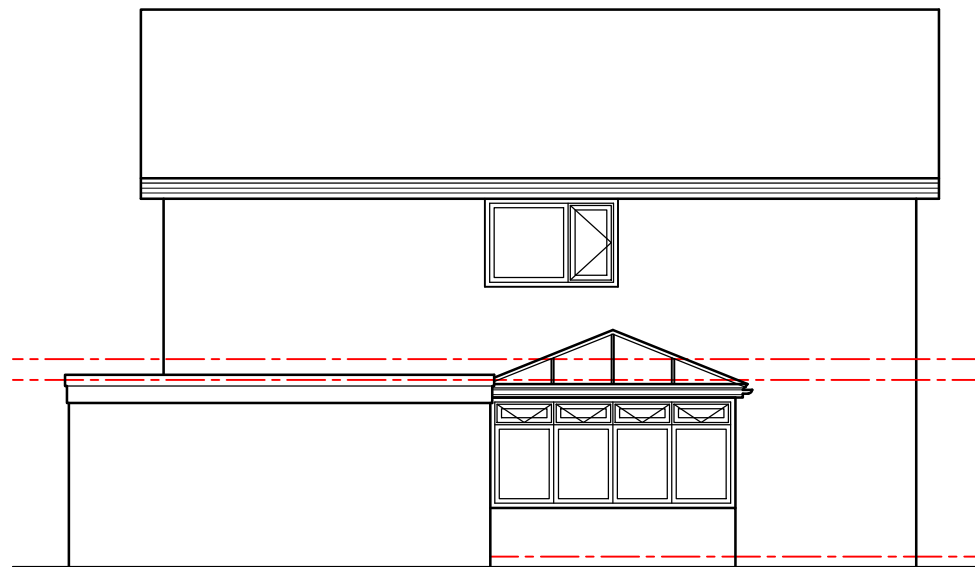
Side 02 Elevation
