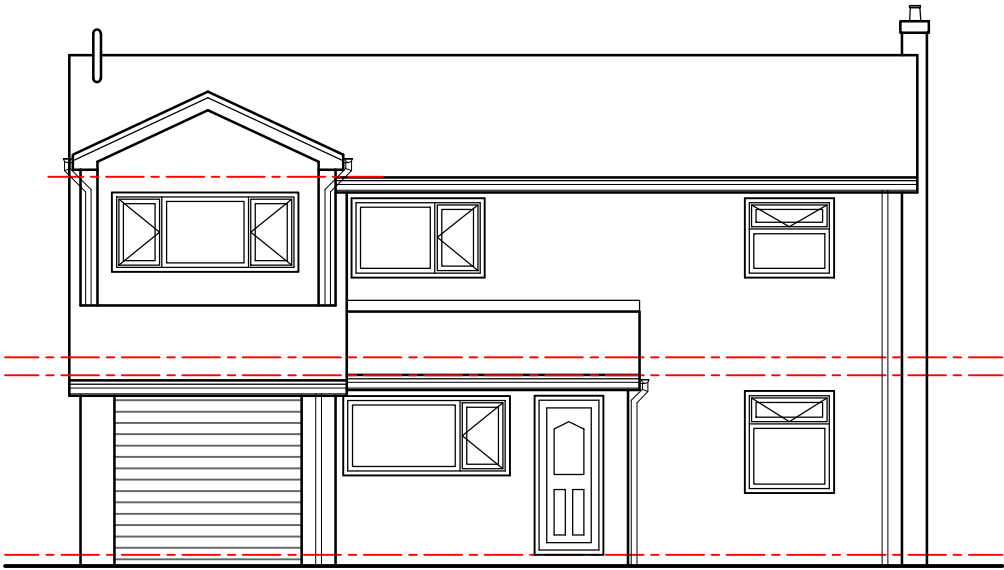
Front Elevation
