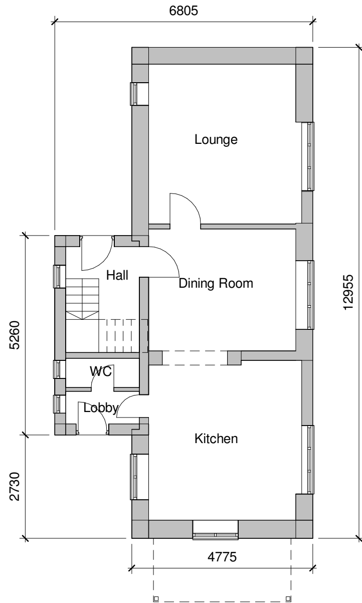
Ground Floor 1 : 100
