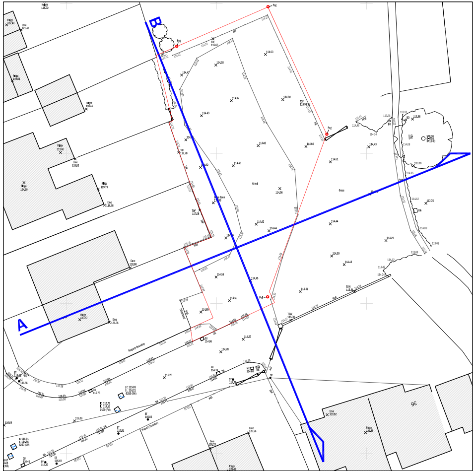
EXISTING SITE KEY PLAN SCALE 1:500
