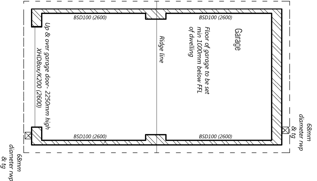
Floor Layout Plan single
