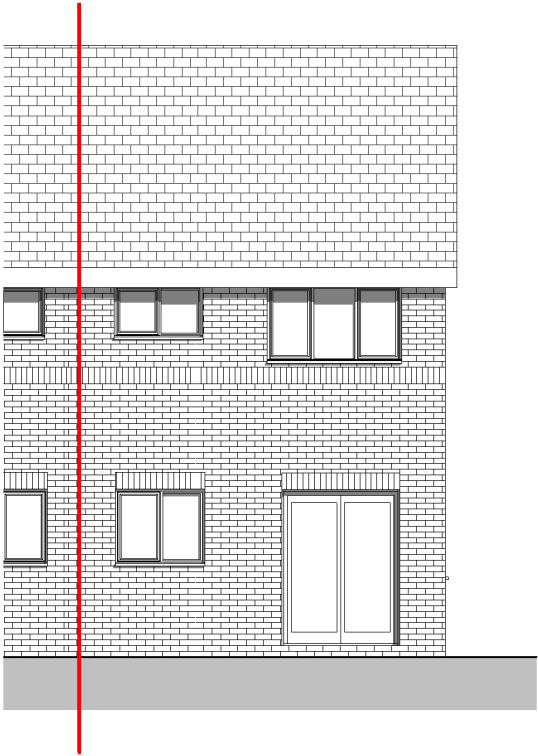
Rear Elevation 1 : 100
