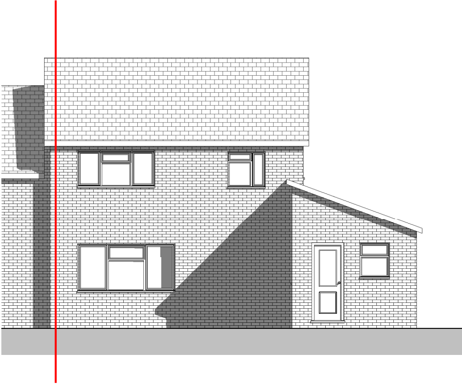
Rear Elevation 1 : 100
