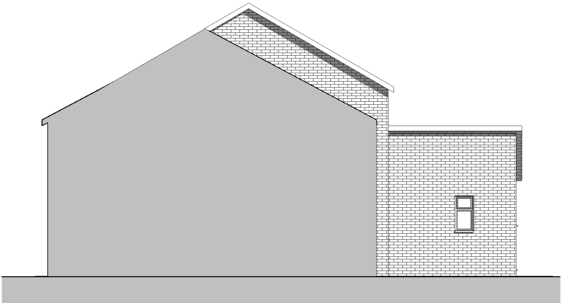
Side Elevation 1 : 100
