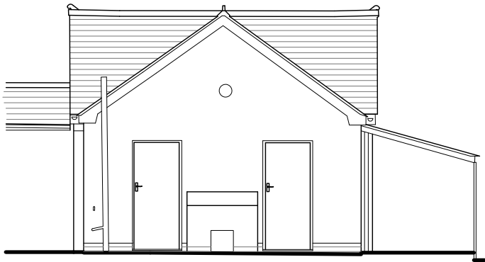
GARAGE NORTH ELEVATION
