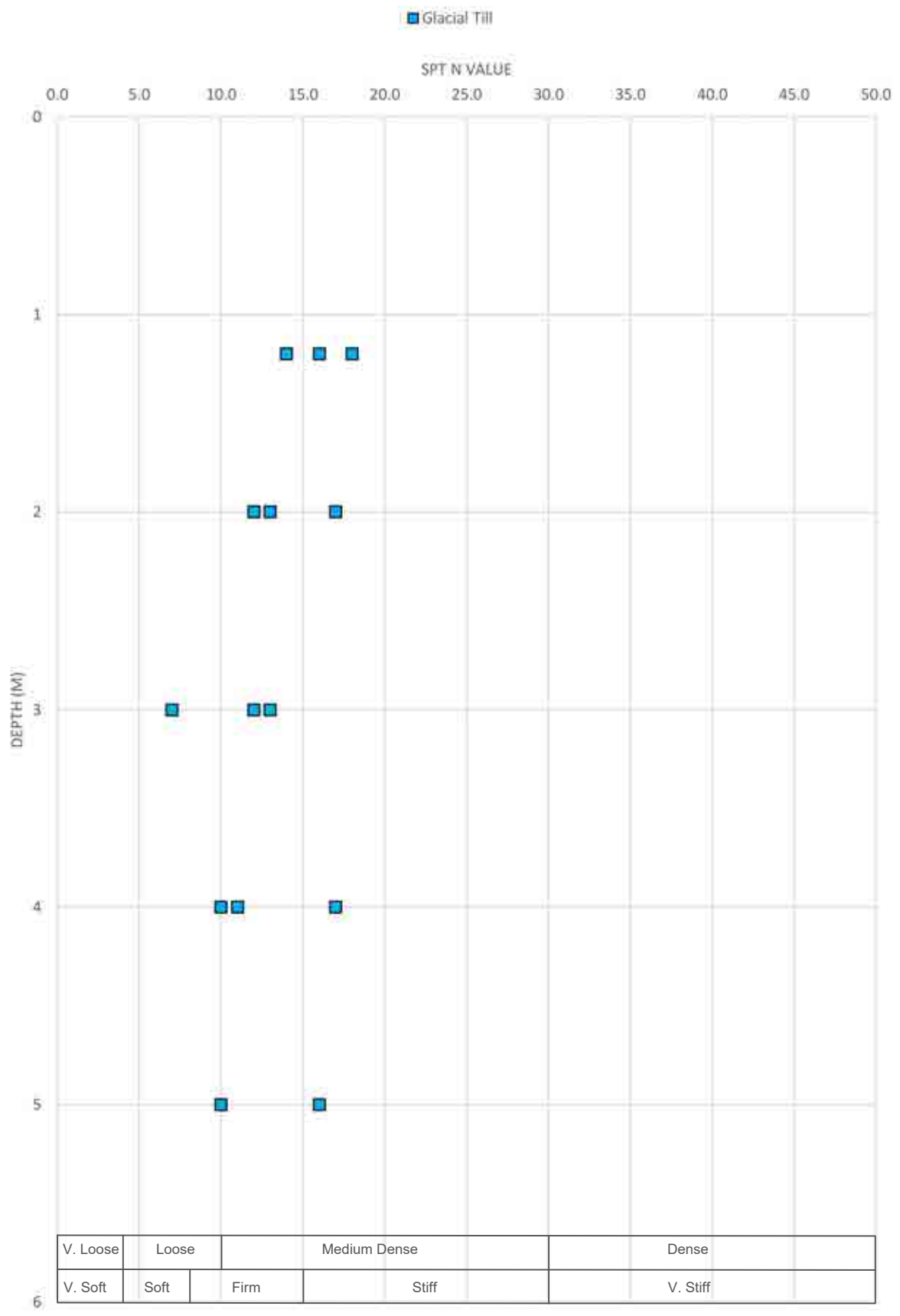
Figure Title SPT 'N' Value Vs Depth FIGURE 5
