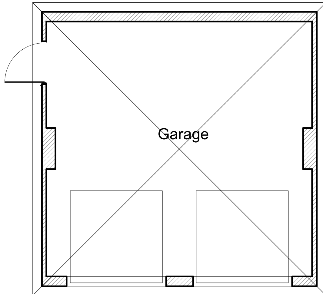
Floor Plan
