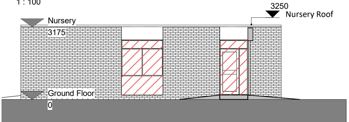
PL - Existing North East Nursery Elevation
