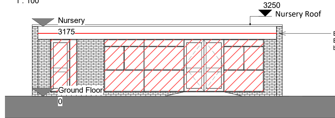
PL - Existing North West Nursery Elevation
