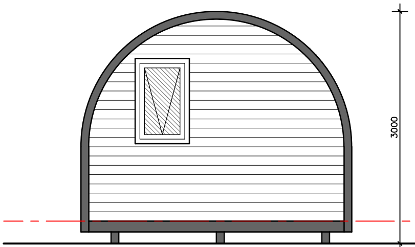
Rear Elevation
