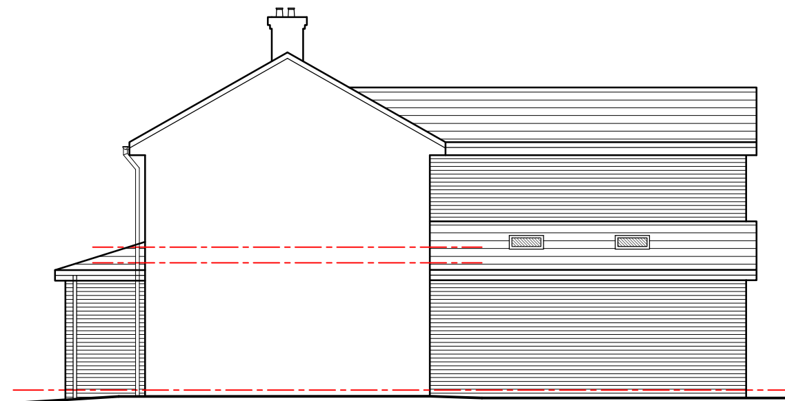
Side Elevation-02
