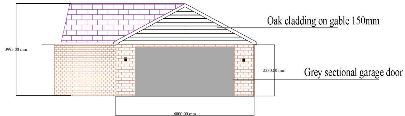
North Elevation
