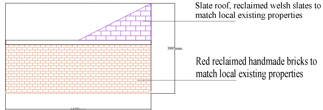
South Elevation
