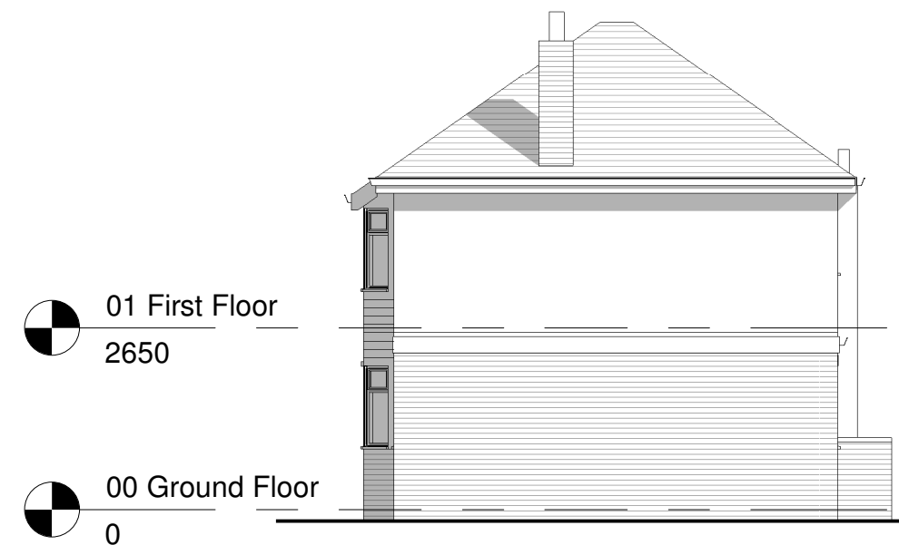
Existing West Elevation 1 : 100
