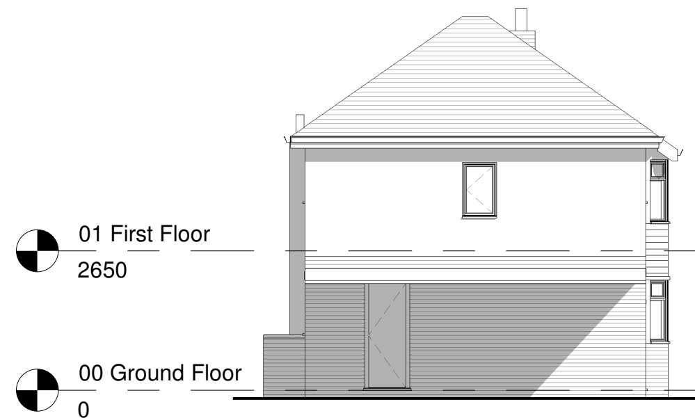
Existing East Elevation 1 : 100
