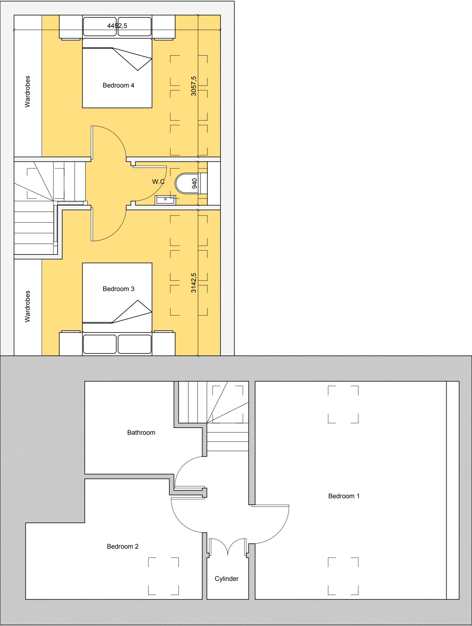
First Floor
