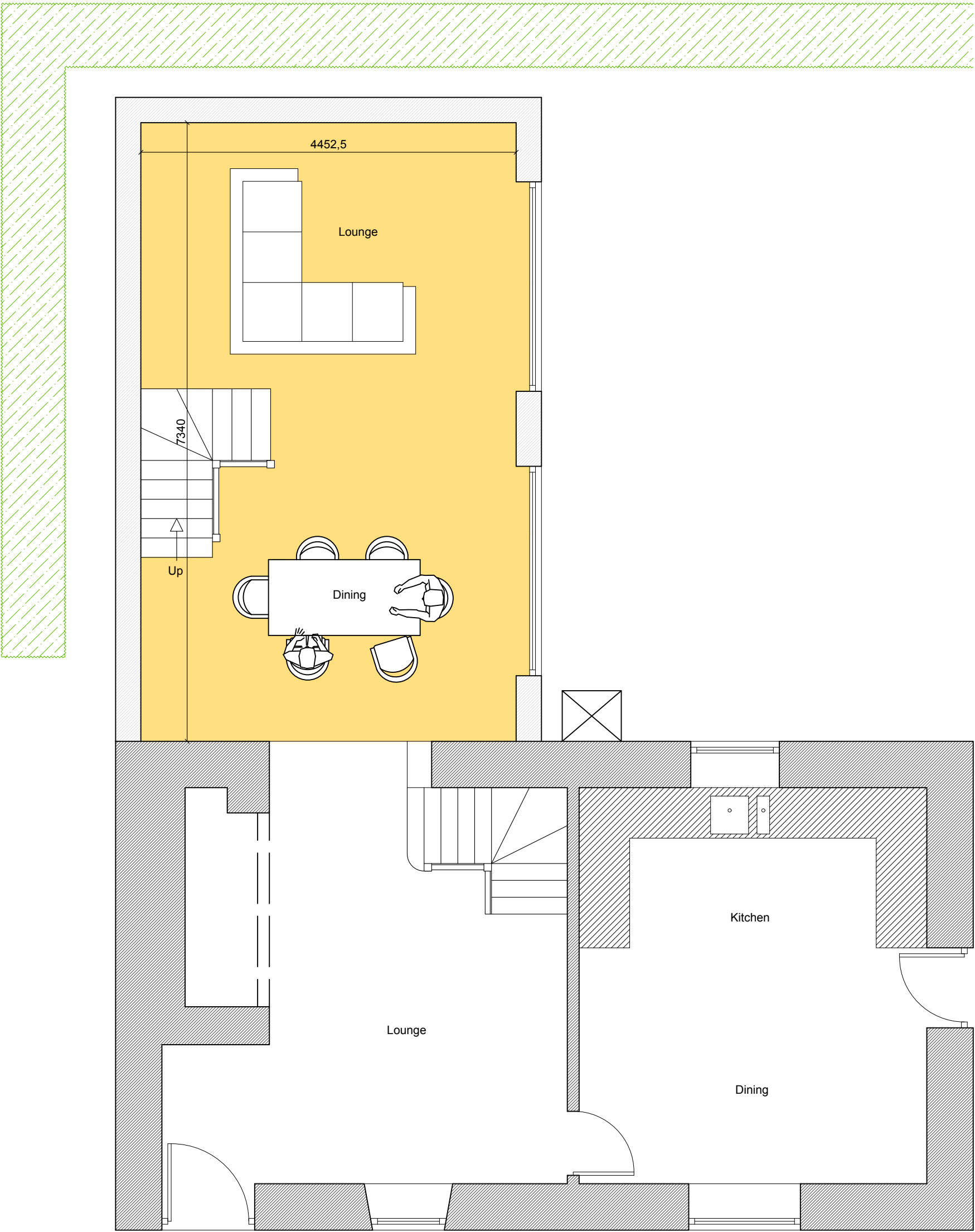
Ground Floor
