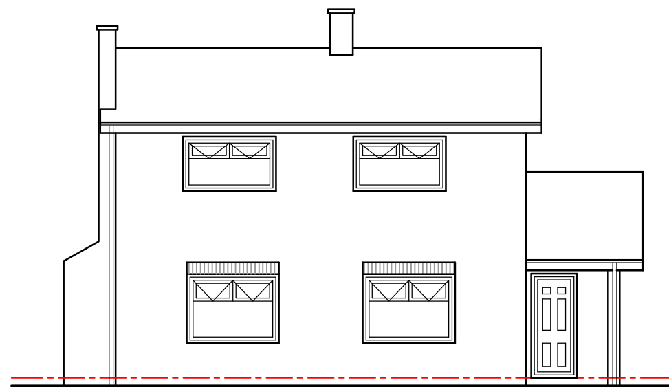
Front Elevation
