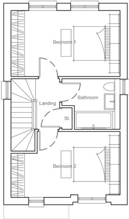
FIRST FLOOR 39.86 sqm
