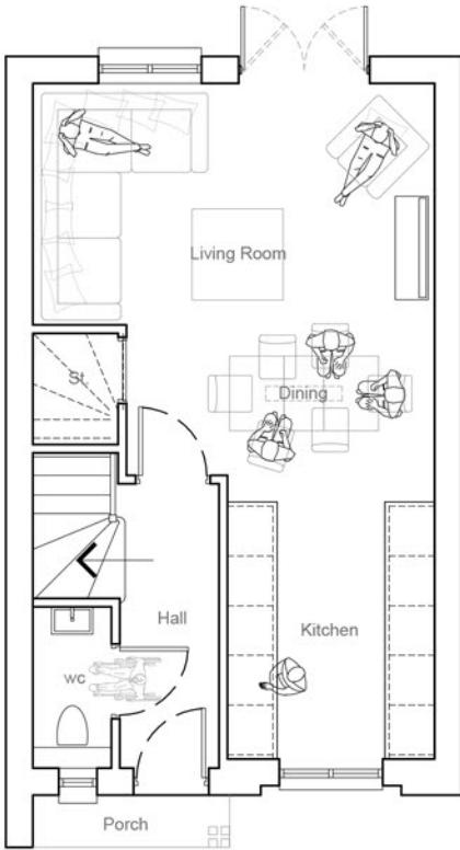
GROUND FLOOR TYPE G 39.81 sqm
